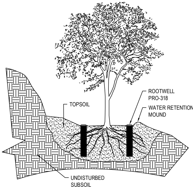
SECTION VIEW
