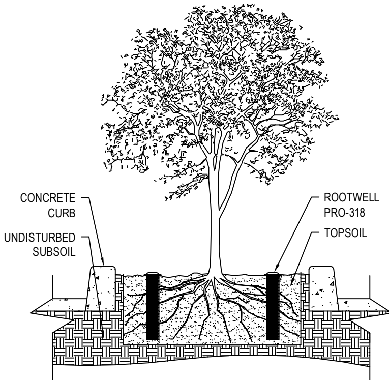
SECTION VIEW
