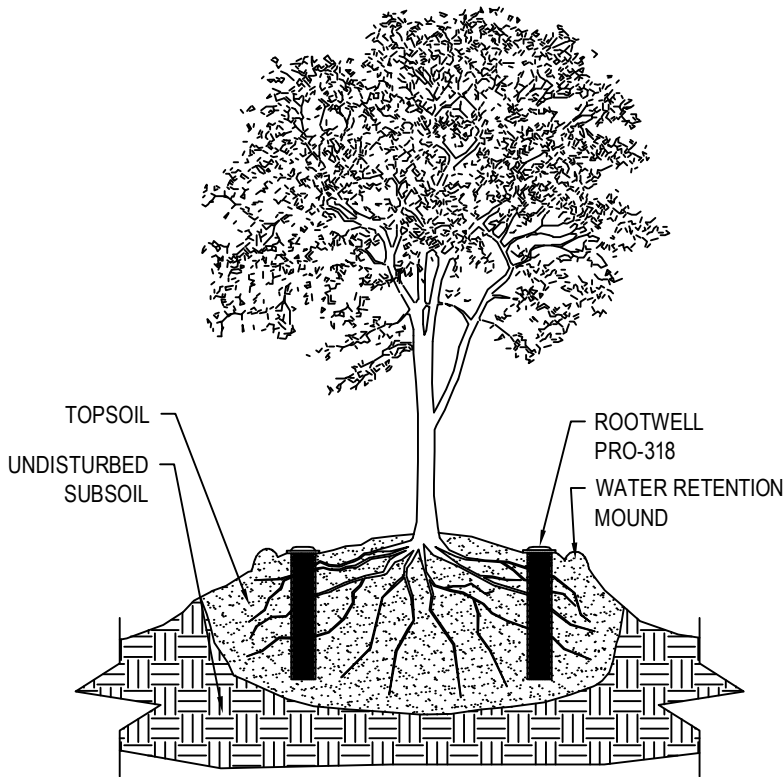
SECTION VIEW
