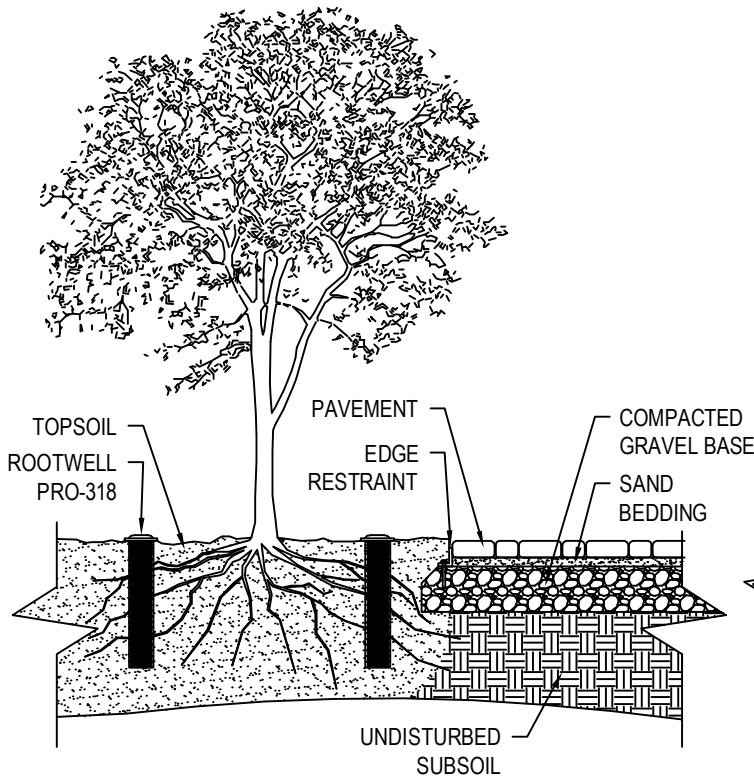
SECTION VIEW
