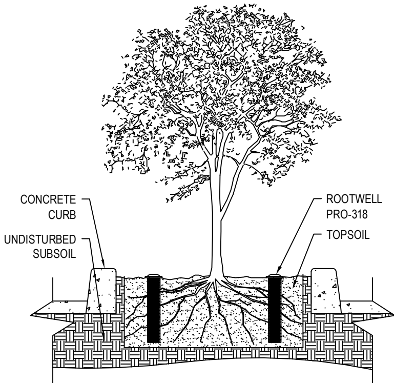
SECTION VIEW
