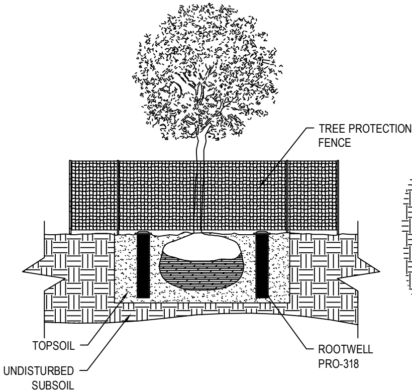
SECTION VIEW
